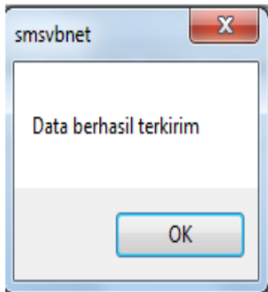
Gambar 13 Report Pesan
